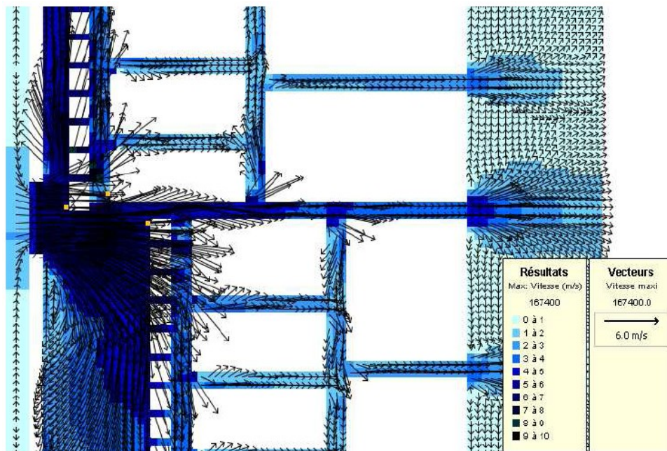
Cas 1 – charge = 5m – vitesses maximales
